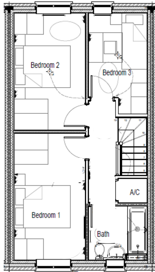
3 Bedroom Floor Plan
