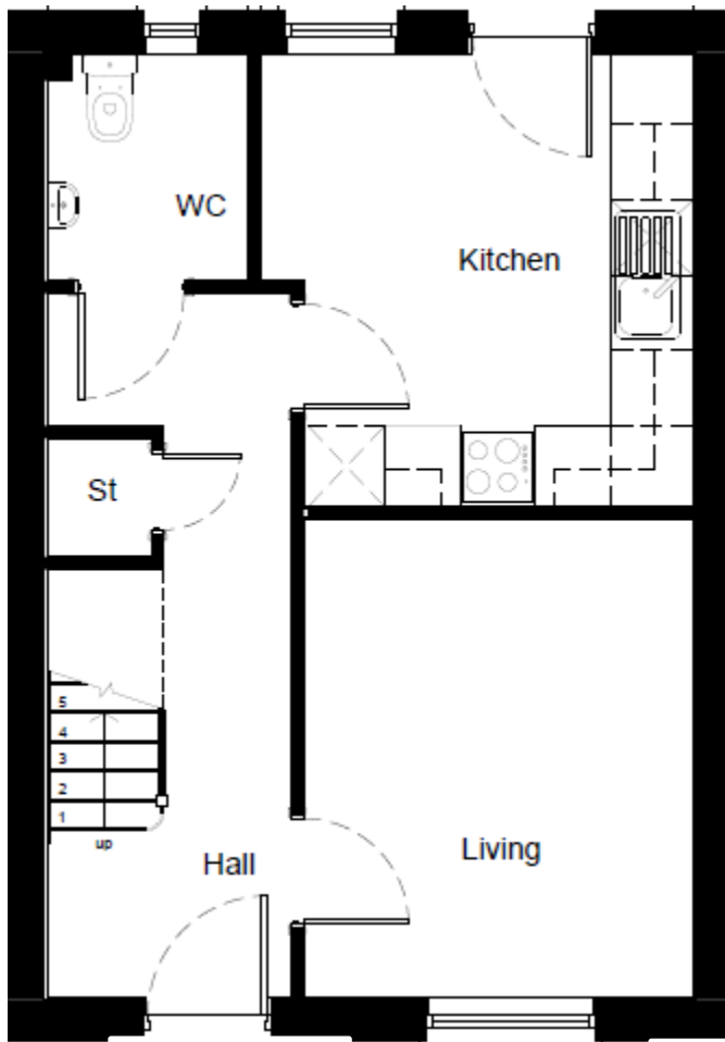
2 BEDROOM FLOORPLAN
