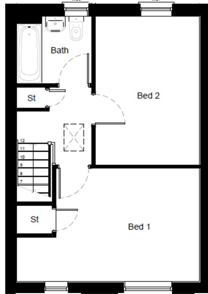
2 BEDROOM FLOORPLAN
